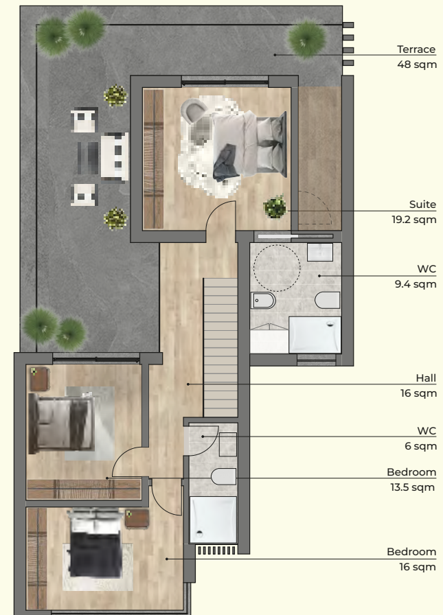
1st Floor
