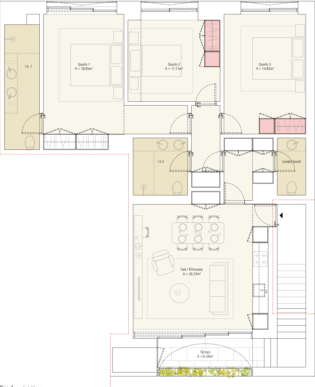
Piso 1 . 1st Floor
