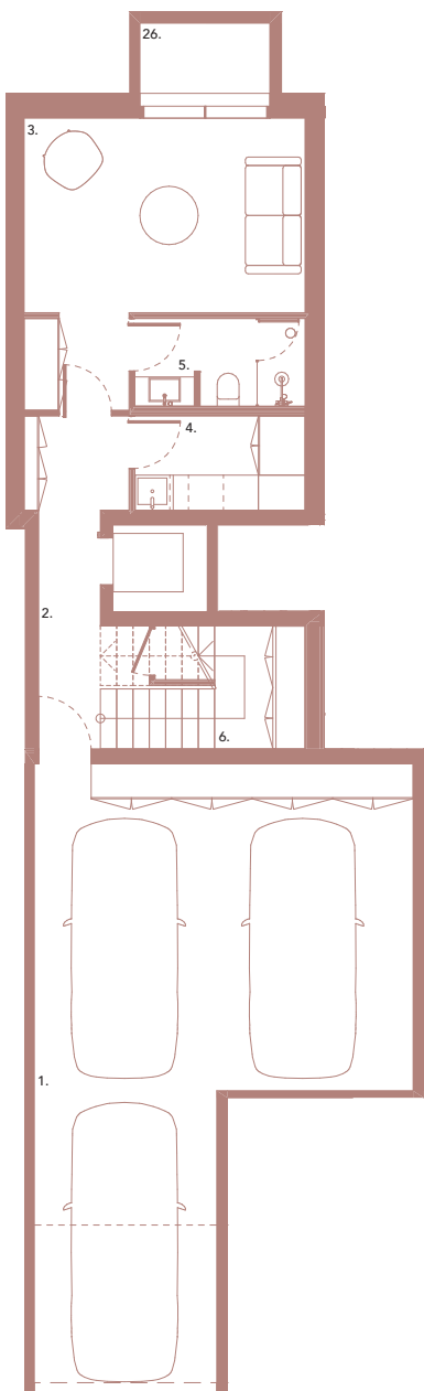
PISO -1 BASEMENT 1
