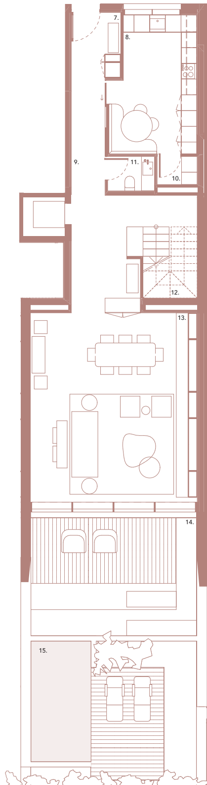
PISO 1 1ST FLOOR
