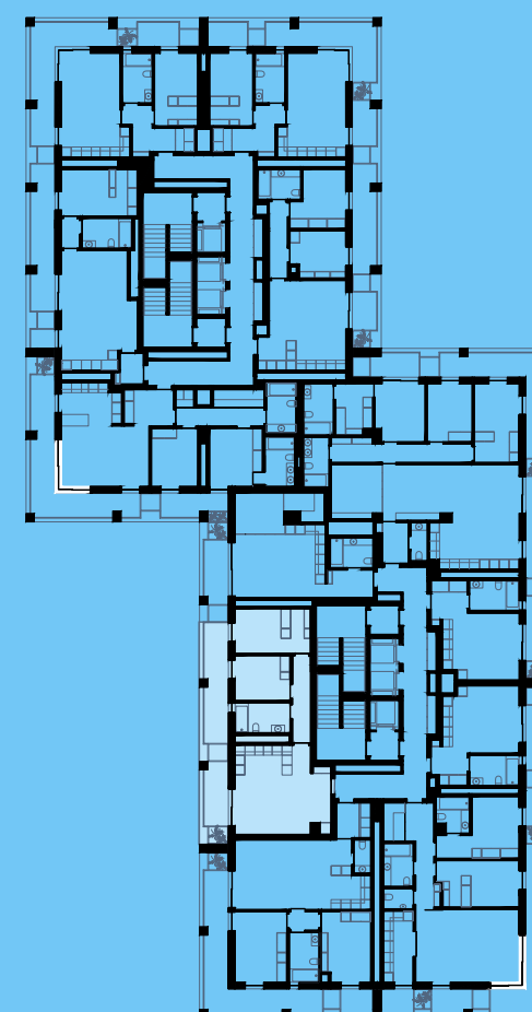
PLANTA PISO 5 | FLOOR PLAN 5
