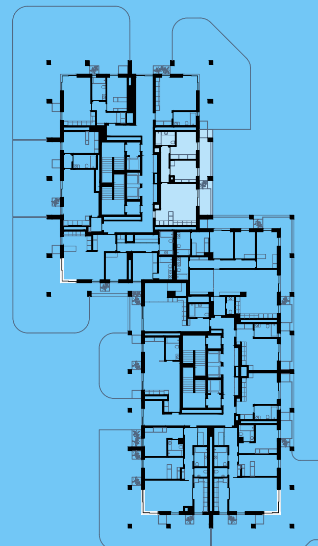
PLANTA PISO 4 | FLOOR PLAN 4
