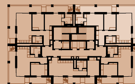
PLANTA PISO 11 | FLOOR PLAN 11
